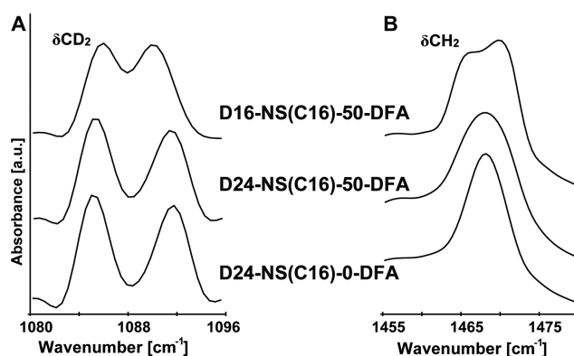
Figure 9. SC models with CER NS acyl chains and FA(C24) chains deuterated at 10 °C. (A) \delta CD 2 mode; a strong peak splitting indicates a strong CD 2 -CD 2 interaction, while weak splitting indicates extensive CD 2 -CH 2 . (B) \delta CH 2 modes of the models; single peak implies limited CH 2 -CH 2 interaction, while the increased peak width indicates a greater CH 2 -CH 2 interaction.
