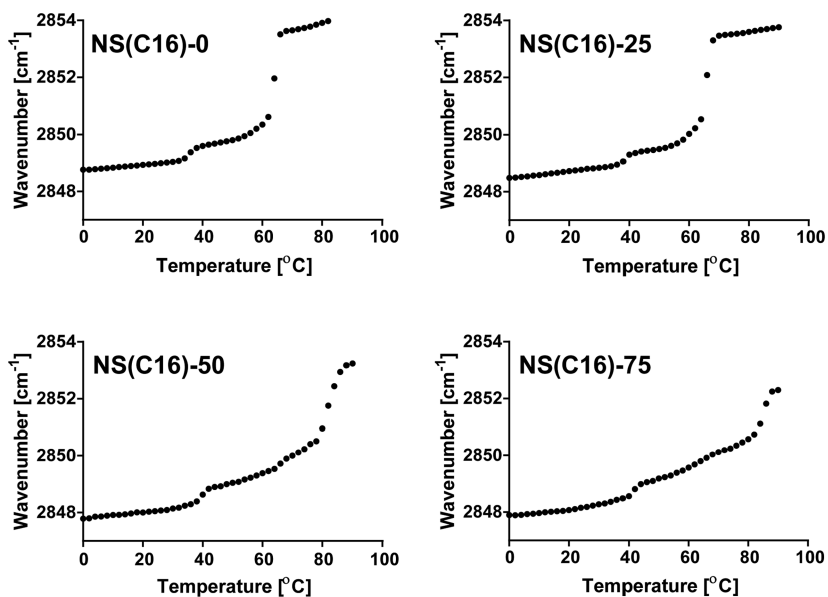
Figure 3. Temperature dependence of the \nu_s\text{CH}_2 mode frequency of the lipid mixtures. The \nu_s\text{CH}_2 modes of all models between 0 and 90 °C, showing initial frequencies below 2850 \text{cm}^{-1} and two distinct phase transitions as temperature increases. Depending on the composition, T_{\text{M,OR-HEX}} was between 34 and 44 °C and T_{\text{M,HEX-LIQ}} was between 60 and 86 °C.
