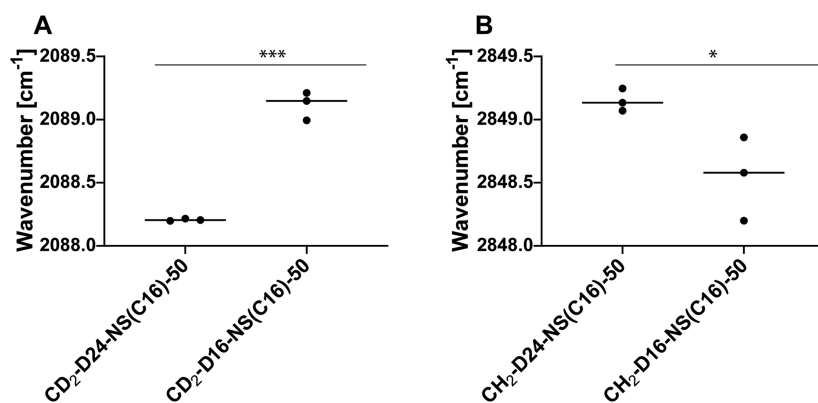
Figure 7. Thermotropic response of NS(C16)-50 \nu_s CH 2 and \nu_s CD 2 frequencies when either C16 or C24 chains are deuterated and the wavenumbers at 10 °C. (A) Wavenumbers at 10 °C for CD 2 -D24-NS(C16)-50 and CD 2 -D16-NS(C16)-50, with C24 and C16 acyl chains deuterated, respectively. The wavenumber of the CER NS(C16) chain is significantly higher than that of the CER NS(C24) chain. (B) Wavenumbers at 10 °C for CH 2 -D24-NS(C16)-50 (arising from protiated chains when only NS(C24) acyl chains are deuterated) and CH 2 -D16-NS(C16)-50 modes (arising from protiated chains when only NS(C16) acyl chains are deuterated). Wavenumber of CH 2 -D24-NS(C16)-50 containing the protiated CER NS(C16) chain is significantly higher than that of the CH 2 -D16-NS(C16)-50 mode in which CER NS(C24) chains were protiated.
