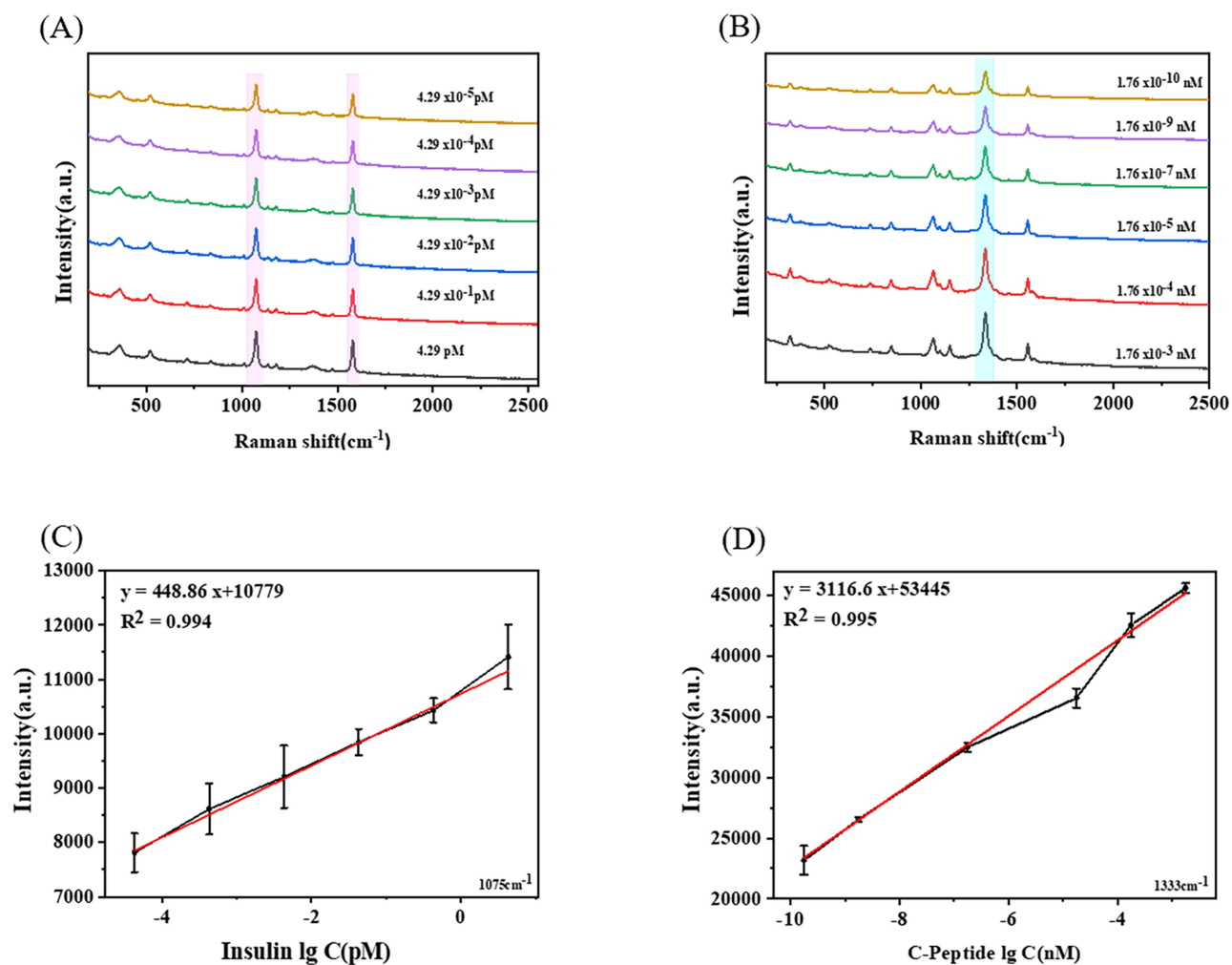
Figure 2 (A) SERS spectrum of Au NRs@4-MBA@SiO 2 @Ag@insulin antibody response to different concentrations of insulin (4.29 pM, 0.429 pM, 4.29 × 10 -2 pM, 4.29 × 10 -3 pM, 4.29 × 10 -4 pM, 4.29 × 10 -5 pM); (B) SERS spectrum of Au NRs@DTNB@SiO 2 @Ag @C-peptide antibody response to different concentrations of C-peptide (1.76 × 10 -3 nM, 1.76 × 10 -4 nM, 1.76 × 10 -5 nM, 1.76 × 10 -7 nM, 1.76 × 10 -9 nM, 1.76 × 10 -10 nM); (C) The calibration curve of peak intensity at 1075 cm -1 varies with the lg value of insulin concentration; (D) Calibration curve of peak intensity at 1333 cm -1 varies with lg value of C-peptide concentration.
