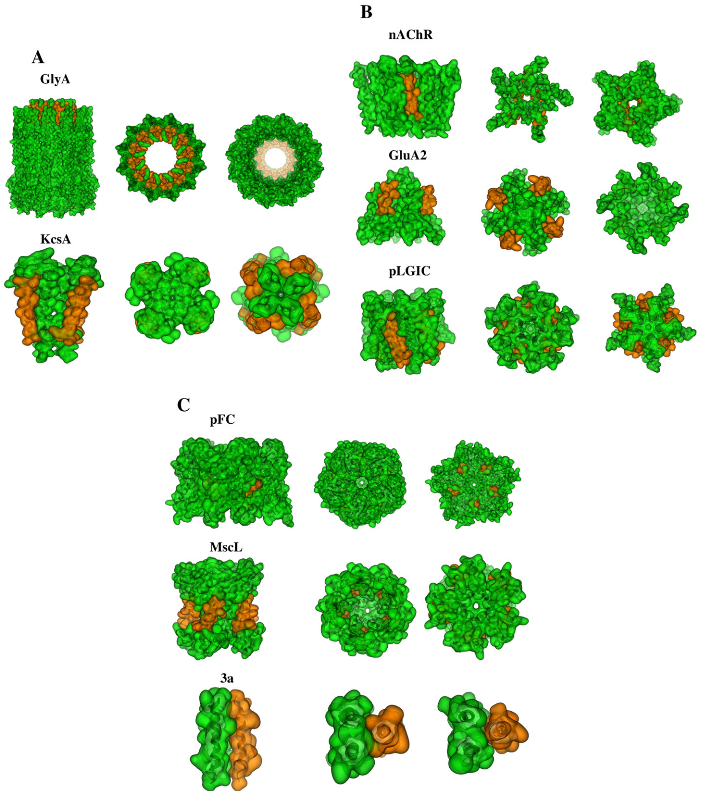
Fig. 3. The toxin ClyA and the channel protein KcsA are shown in a side view (left) and a view from the respective top (middle) and bottom (right) of the protein (A). For the channel proteins only the TMDs are shown. The TMDs of nAChR, GluA2 and pLGIC are shown in the same way (B), so are the TMDs of the formate channel, Mscl and 3a (C). The proteins are shown in green with the helical backbones sketched. Overlapping domains with Vpu 6–27 are highlighted in orange.
