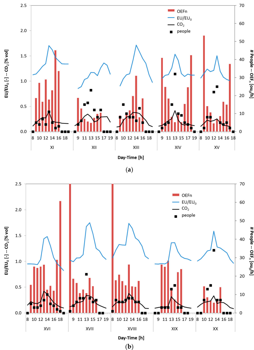
Figure 6. Trends of EU/EU_0 , CO_2 concentration, number of occupants and estimated OEF_n for the period from day XI to XV (a); and for the period from day XVI to XX (b).
