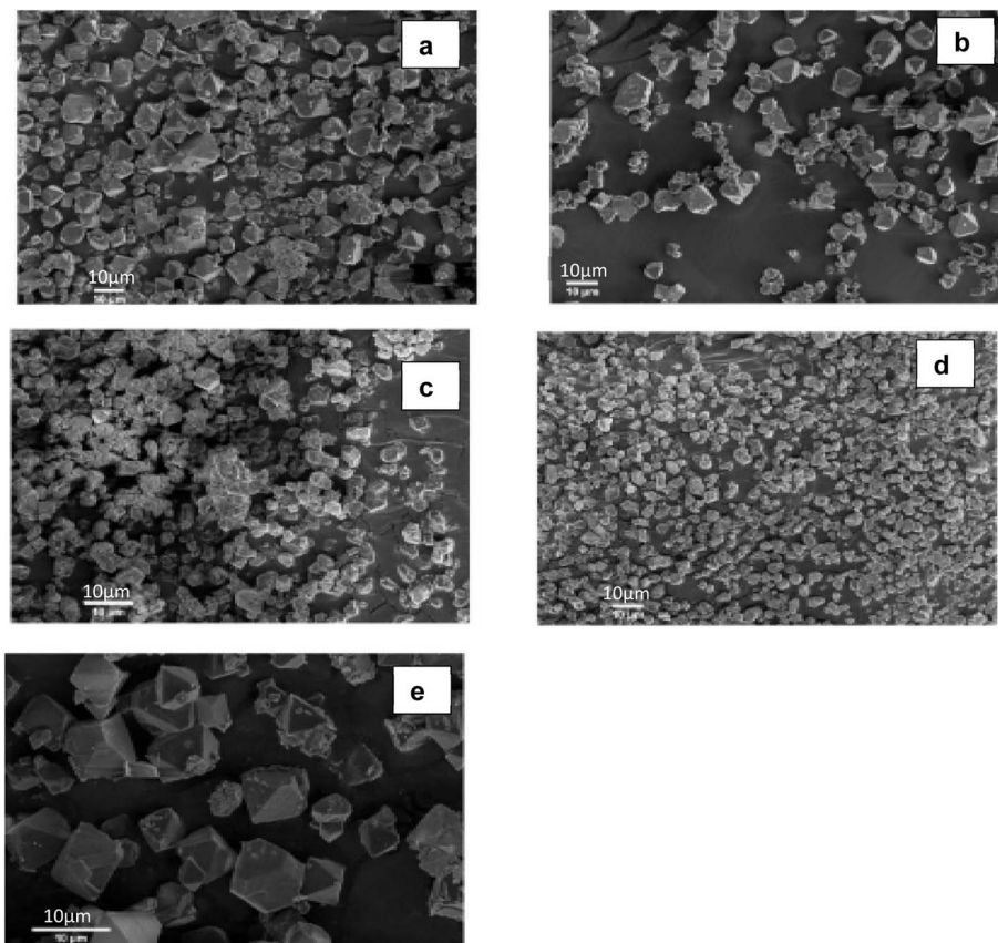
Fig. 11 SEM analysis of produce Cu-BTCs under various solvent mixture (a) H 2 O–DMF, (b) H 2 O–ethanol–DMF, (c) H 2 O–ethanol–NaOH, (d) H 2 O–ethanol–NH 4 OH, and (e) H 2 O–ethanol–primidine. Reproduced from Israr et al. 89 with permission from Elsevier, copyright 2016.
