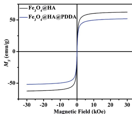
Fig. 5 Magnetization curves of \text{Fe}_3\text{O}_4@HA and \text{Fe}_3\text{O}_4@HA@PDDA NPs.
