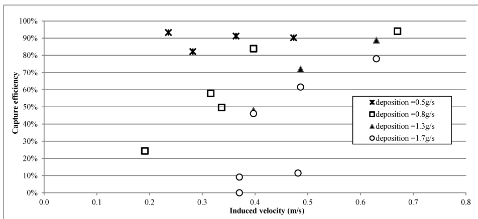
Figure 8 Capture efficiencies with respect to induced velocity for different deposition rates ( 30^\circ inclination, 1.0 mm wire).
