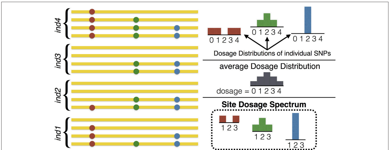
FIGURE 3 | Illustration of the relation between the Dosage Distribution and the Site Dosage Spectrum. On the left, homologous sequences from 4 tetraploid individuals are shown ( n = 4, p = 4 ), containing 3 SNPs of frequency 50%. On the right, the three DDs (one for each SNP) are shown at the top. The SDS at the bottom is the distribution of these DDs (which in this example is given by the three DDs with probability 1/3 each). Note that the SDS bears no relation with the average DD, which is shown in the middle. In this example, the Site Frequency/Dosage Spectrum would be \psi_{8, \{1/4, 0, 1/4\}} = 1/3 , \psi_{8, \{1/4, 1/2, 1/4\}} = 1/3 , \psi_{8, \{0, 1, 0\}} = 1/3 and \psi_{8, \{I\}} = 0 for other choices of I .
