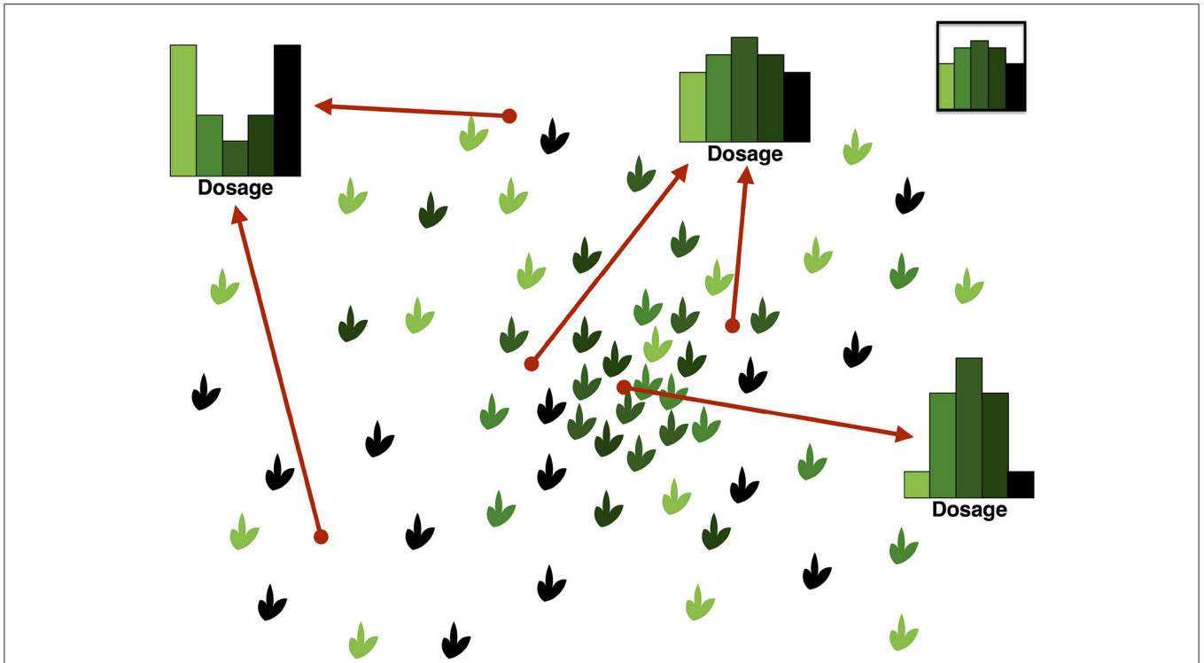
FIGURE 2 | Illustration of the Dosage Distribution (including homozygotes) in a panmictic autotetraploid population with density-dependent selfing rates. In this example, we assume for simplicity that segregating alleles are at intermediate frequency in the population; their dosage in each individual is represented by the color lightness. Since the average frequency is the same everywhere, the average dosage also is. However, by contrast, the DD depends strongly on the sampling location because of variations in the local spatial density. Sampling individuals at random across different locations would result in an average DD like the one in the top-right inset. On the other hand, sampling around a given location would result in different DDs, as illustrated. Locations in the central region tend to have DDs similar to the Hardy–Weinberg ones, while peripheral locations show a large excess of homozygotes because of sampling.
