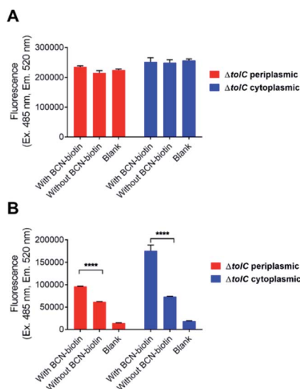
Fig. 5 Tetrazine dye 2 detection of BCN biotin 1 . \Delta\text{TolC} E. coli were incubated in media supplemented with (A) or without glucose (B) before the addition of L -rhamnose with or without 40 \mu\text{M} BCN-biotin 1 . Cells were lysed with MeCN containing 2 \mu\text{M} tetrazine-BDP-FL 2 and allowed to react for 1 hour at room temperature and then clarified for fluorescence measurement. A blank control was prepared without BCN-biotin 1 and tetrazine-BDP-FL 2 . Data was analysed using a two-way ANOVA test followed by Tukey's multiple comparison post hoc test ( n = 3 , mean \pm SD, * p < 0.05 , ** p < 0.01 , *** p < 0.001 , **** p < 0.0001 ).
