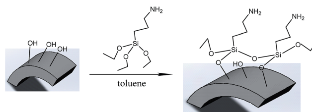
Scheme 5 The binding mechanism between APTES and the \alpha -Al 2 O 3 support surface.
