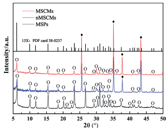
Fig. 2 XRD patterns of the nMSCMs, MSCMs and MSPs. ◆: \alpha -Al 2 O 3 ; ○-13X molecular sieve.
