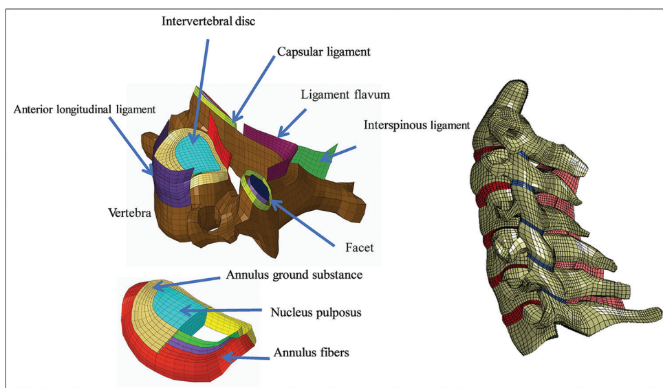
Figure 1: Finite-element model with the details of components. See text for details
