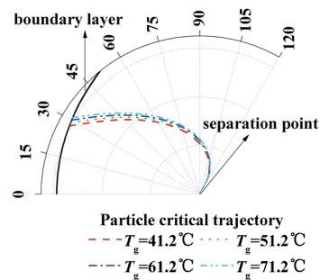
Fig. 6 Critical removal trajectory of particle ( d_p = 1 \mu\text{m} ) in thermal boundary layer along a single film with different temperature gradient and same humidity gradient ( T_w = 5^\circ\text{C} ).
