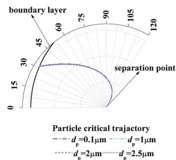
Fig. 7 Critical removal trajectory in the thermal boundary layer along a single water film for different particle sizes ( T_g = 41.2^\circ\text{C} , \phi_g = 0.85 , T_w = 5^\circ\text{C} ).
