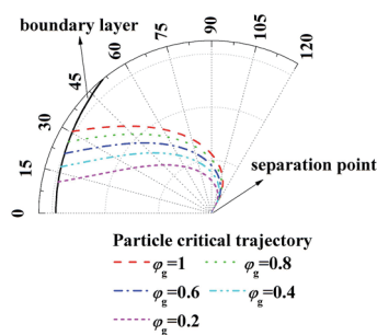
Fig. 5 Critical removal trajectory of particle ( d_p = 1 \mu\text{m} ) in thermal boundary layer along a single film with different humidity gradient and same temperature gradient ( T_g = 41.2^\circ\text{C} , T_w = 5^\circ\text{C} ).
