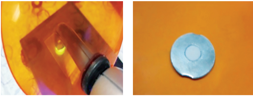
Figure 2 - Composite disc preparation.
