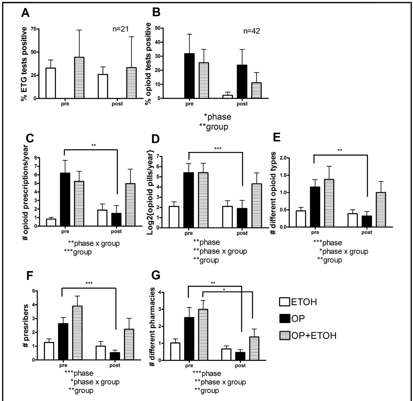
FIGURE 1. Urine drug test results (A and B), PDMP measures of opioid prescribing activity (C–E) and health care system involvement (F and G) pre versus post initial injection. (A) Percent of positive ETG tests trended downward non-significantly among the n = 21 subjects (ETOH, n = 18 ; OP + ETOH, n = 3 ) that had ETG testing both before and after initial INTX injection. (B) Percent of positive opioid tests differed by group and decreased post-injection among the n = 42 subjects (ETOH, n = 22 ; OP, n = 11 ; OP + ETOH, n = 9 ) that had opioid testing both before and after initial INTX injection (ETOH: Patients with alcohol without opioid use disorders; OP: patients with opioid but not alcohol use disorders; OP + ETOH patients with both alcohol and opioid use disorders). For all PDMP data (C–G) all N = 68 subjects are shown graphically and included in the statistical analysis. (C) The number of opioid prescriptions (adjusted to annual rates), differed between groups and dropped specifically in the OP group. (D) Annual adjusted numbers of opioid doses (normalized by Log base 2 transformation), differed by group, dropped overall, and in a significantly more robust way for the OP group. (E) Number of different types of opioids dispensed also differed by group, dropped overall, and in a more robust way for the OP group. (F) The number of prescribers dispensing controlled substances, differed by group, dropped overall, and in a significantly more robust way for the OP group. (G) The number of pharmacies dispensing controlled substances, differed by group, dropped overall, and in a significantly robust way for the OP and the OP + ETOH groups. Bars show means \pm SEMs. Significant results from ANOVAs are noted where they occur ( *p < .05 ; **p < .01 ; ***p \leq .001 ).
