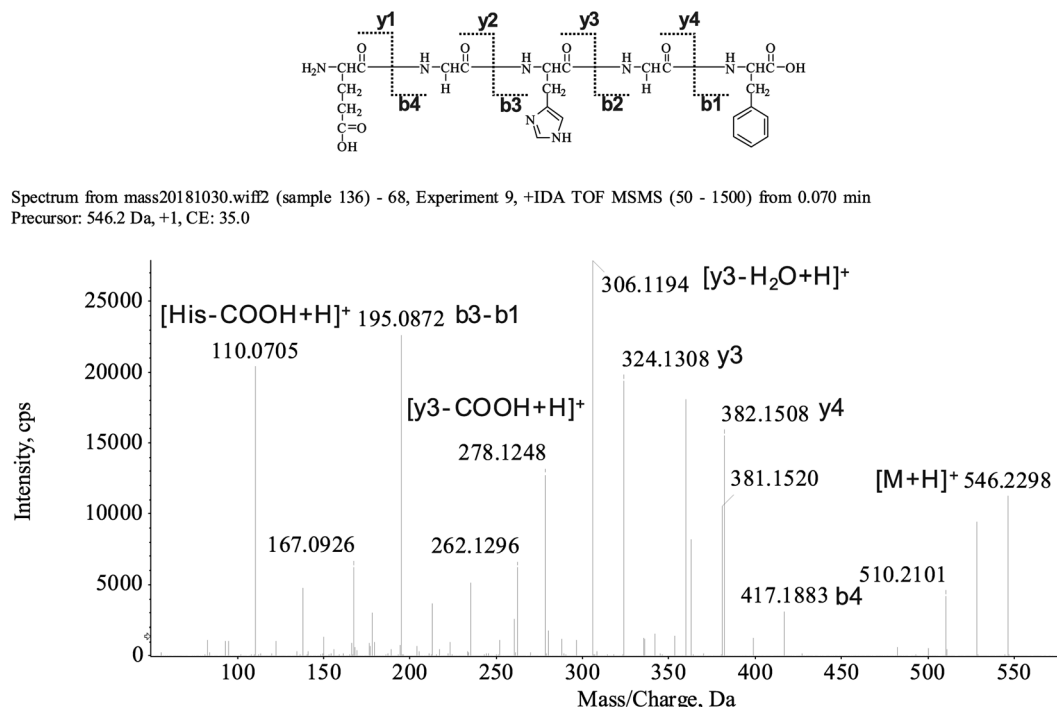
Fig. 2 MS spectrum and structure of LZO-3.
