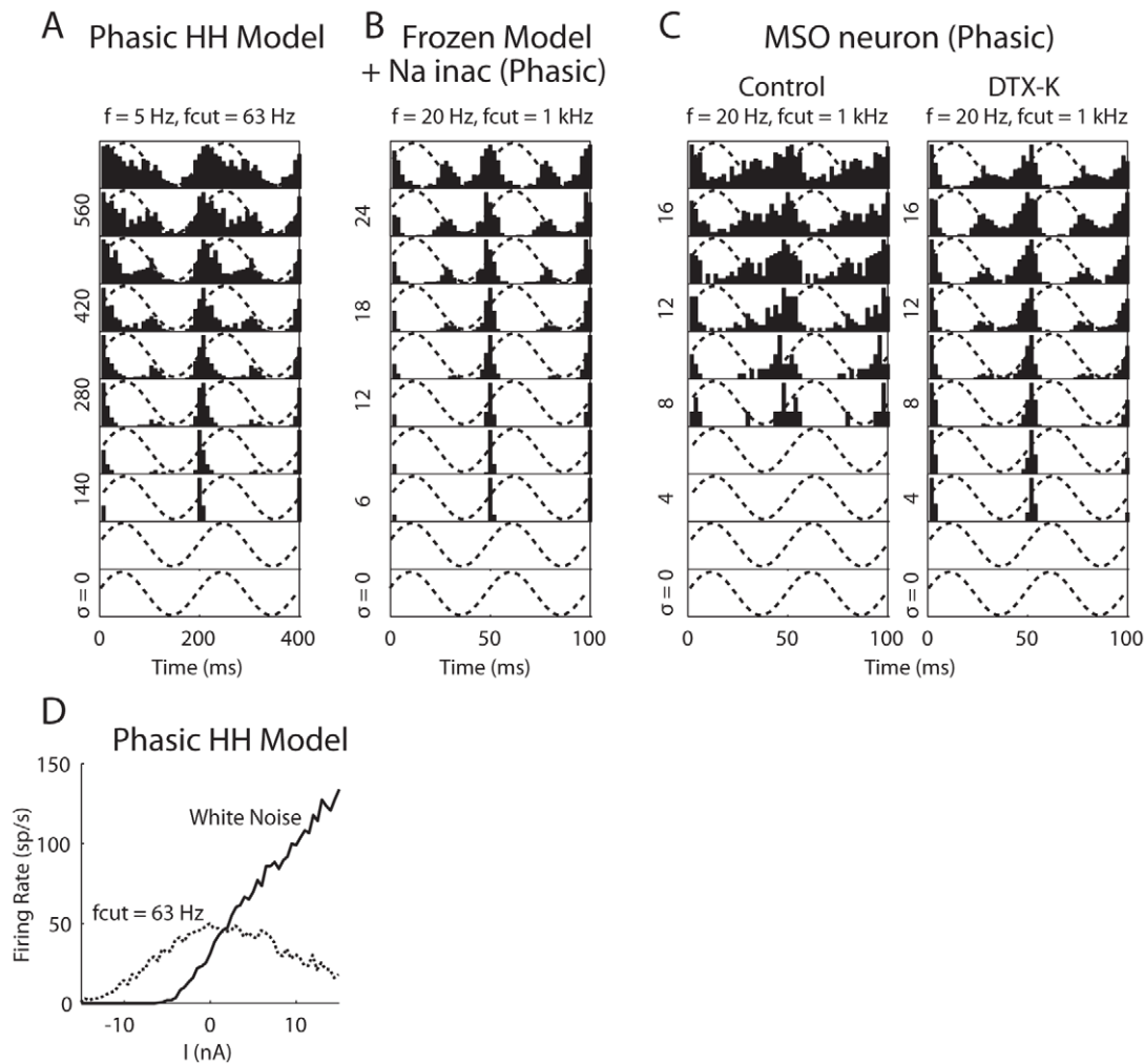
Figure 10. Responses of other models and neuron to a subthreshold signal with noise. (A–C) Period histograms in response to subthreshold signals with different amount of noise added. (A) The phasic Hodgkin and Huxley (HH) model (Clay et al. 2008) at 18.5°C. The signal was a sinusoid with A_s = 15 nA/cm 2 . (B) A new phasic model created from the tonic model ( I_{KLT} was frozen) by shifting the voltage dependency of the sodium inactivation by -15 mV at 32°C. The signal was a sinusoid with A_s = 2 nA. (C) An MSO neuron recorded in a brain slice from a gerbil aged P18 before and after 60 nM DTX-K was bath applied at 32°C. The signal was a modified sinusoid (the negative part of the sinusoid was multiplied by a factor of 0.5) with A_s = 1.5 nA. The dotted lines are superimposed signals scaled to illustrate the response phase. (D) f - I curves of the phasic HH model obtained with white noise ( \sigma = 100 pA/cm 2 ) and low-pass filtered noise ( \sigma = 500 pA/cm 2 ). f_s signal frequency. f_{cut} cutoff frequency of the low-pass filtered noise. Noise \sigma [in pA/cm 2 in (A) and pA in (B) and (C)] is measured with the white noise before low-pass filtering. doi:10.1371/journal.pcbi.1000825.g010
