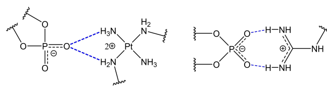
Scheme 2. Structural representation of salt bridge interactions with phosphodiesters by cationic platinum complex (left), and guanidiniums (right).
