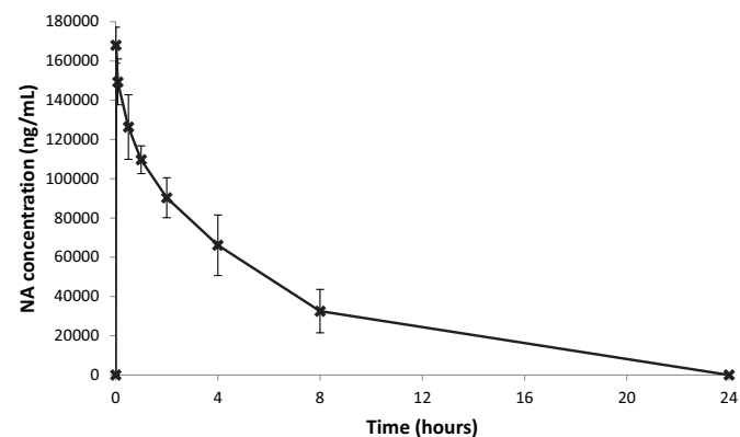
Fig. 1. Mean concentrations of NA in the plasma of male rats (n = 3) following a single IV dose at a nominal dose level of 120 mg/kg (group A).
