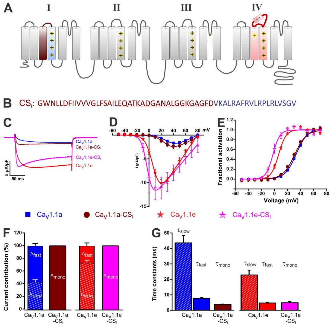
Figure 3. Insertion of IS3 with the IS3-S4 linker of Ca_V1.2 into the I VSD of Ca_V1.1a and Ca_V1.1e alters kinetics but not the voltage dependence or amplitude. (A) Transmembrane topology of Ca_V1.1 indicating the insertion of the Ca_V1.2 IS3 helix and the IS3-S4 linker (brown) into the corresponding regions of Ca_V1.1 . (B) Amino acid sequence of cardiac S3, S3-S4 linker (brown), and skeletal S4 (blue) in the I repeat VSD. (C) Representative calcium currents at maximal activation of Ca_V1.1a , Ca_V1.1e , Ca_V1.1a-CS_i , and Ca_V1.1e-CS_i . (D and E) I/V curves (D) and fractional activation plots (E) show that neither current density nor voltage sensitivity is significantly affected by insertion of the cardiac IS3 and IS3-S4 linker in Ca_V1.1a or Ca_V1.1e . (F) Transferring the Ca_V1.2 IS3 helix and IS3-S4 linker into Ca_V1.1 gives rise to currents with the activation phase described by a single exponential function. (G) The time constants of the single activation component of Ca_V1.1a-CS_i and Ca_V1.1e-CS_i resemble the fast components of Ca_V1.1a and Ca_V1.1e . Data in graphs represent mean \pm SEM. Numerical values, number of samples, and statistical significance are reported in Tables 1 and 2.
