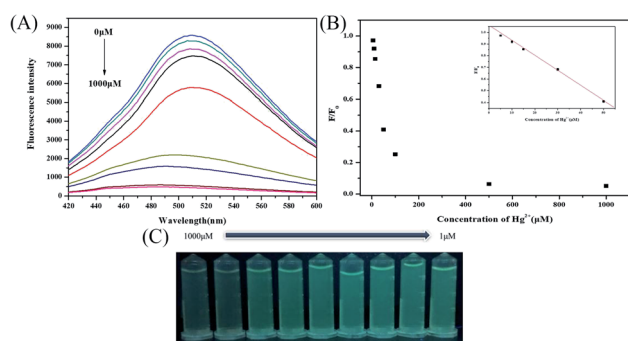
Fig. 5 (A) Change in fluorescence intensity of CDs on adding Hg^{2+} . (B) Linear plotting of F/F_0 versus concentration of Hg^{2+} . (C) Photographs of the corresponding detection condition.
