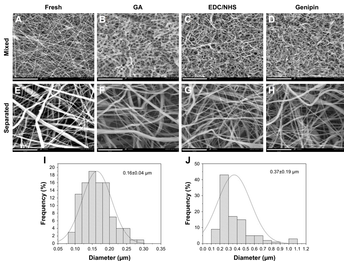
Figure 2 SEM images of different cross-linked membranes under mixed 10% (w/v) solution of PCL/collagen (A–D) and separated 10% (w/v) PCL and 10% (w/v) collagen solution (E–H). (I, J) Fiber diameter distribution of MF and SF, respectively.
