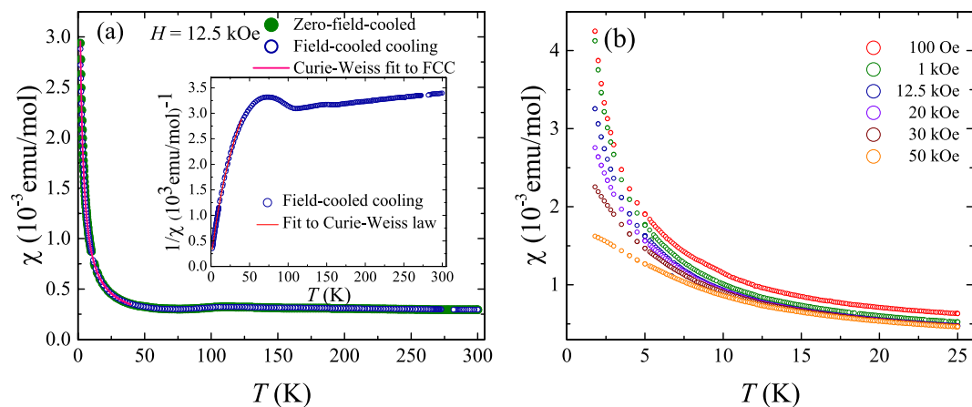
Figure 2. (a) Susceptibility versus temperature and its inverse (inset) for a polycrystalline sample of \text{VSe}_2 . The fit to a modified Curie-Weiss law from 1.8–40 K for both the susceptibility versus temperature and its inverse are also shown. (b) Low-temperature susceptibility for the polycrystalline sample of \text{VSe}_2 at different applied magnetic fields.
