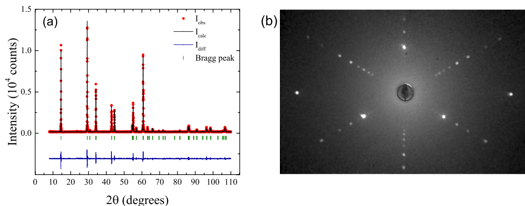
Figure 1. (a) Room temperature powder X-ray diffraction pattern of \text{VSe}_2 . The experimental profile (red closed circles) and a full profile matching refinement (black solid line) made using the P\bar{3}m1 hexagonal structure are shown, with the difference given by the blue solid line. (b) X-ray Laue back scattered diffraction pattern for a single crystal of \text{VSe}_2 viewed along the [001] direction.
