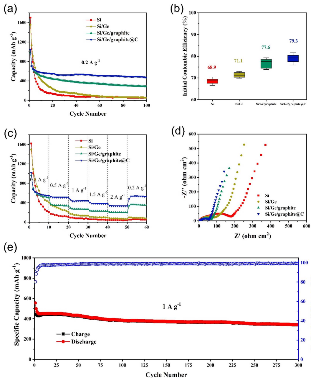
Fig. 5 Comparison of cycling performances at 0.2 A g -1 (a), initial coulombic efficiencies (b), rate performances (c) and Nyquist plots of Si, Si/Ge, Si/Ge/graphite and Si/Ge/graphite@C composites (d), respectively. (e) Long-term cycling performance of Si/Ge/graphite@C at 1.0 A g -1 .
