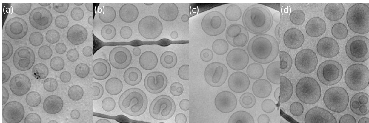
Figure 6. Cryo-TEM images of the produced manganese-loaded NLS and SLL liposomes. LP-NLS-MC (a), LP-NLS-MA (b), LP-SLL-MC (c) and LP-SLL-MA (d). Bar corresponds to 200 nm.
