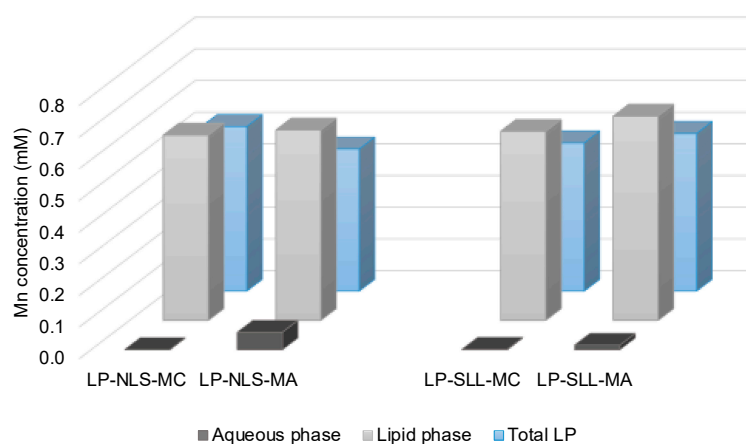
Figure 7. MC and MA concentration in the aqueous phase (dark grey), in the lipid phase (light grey) of LP-NLS and LP-SLL after ultracentrifugation, and in the formulations before ultracentrifugation (light blue). Data are the means of three independent experiments conducted in duplicate.
