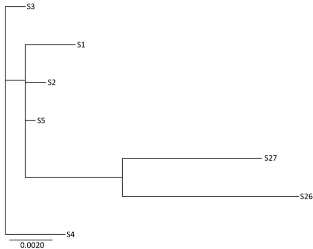
Figure 3. Phylogenetic tree of 7 sequence type 34 Klebsiella pneumoniae isolates tested during phenotypic and genotypic characterization of Enterobacteriaceae producing oxacillinase-48–like carbapenemases, United States. Genetic diversity ranged from 1 to 33 high-quality single-nucleotide polymorphisms that were called in an \approx 5 Mb core genome, which equals \approx 90\% of the reference genome size (isolate 1 sequenced by using Pacific Biosciences [Menlo Park, CA, USA] technology). Scale bar indicates nucleotide substitutions per site.
