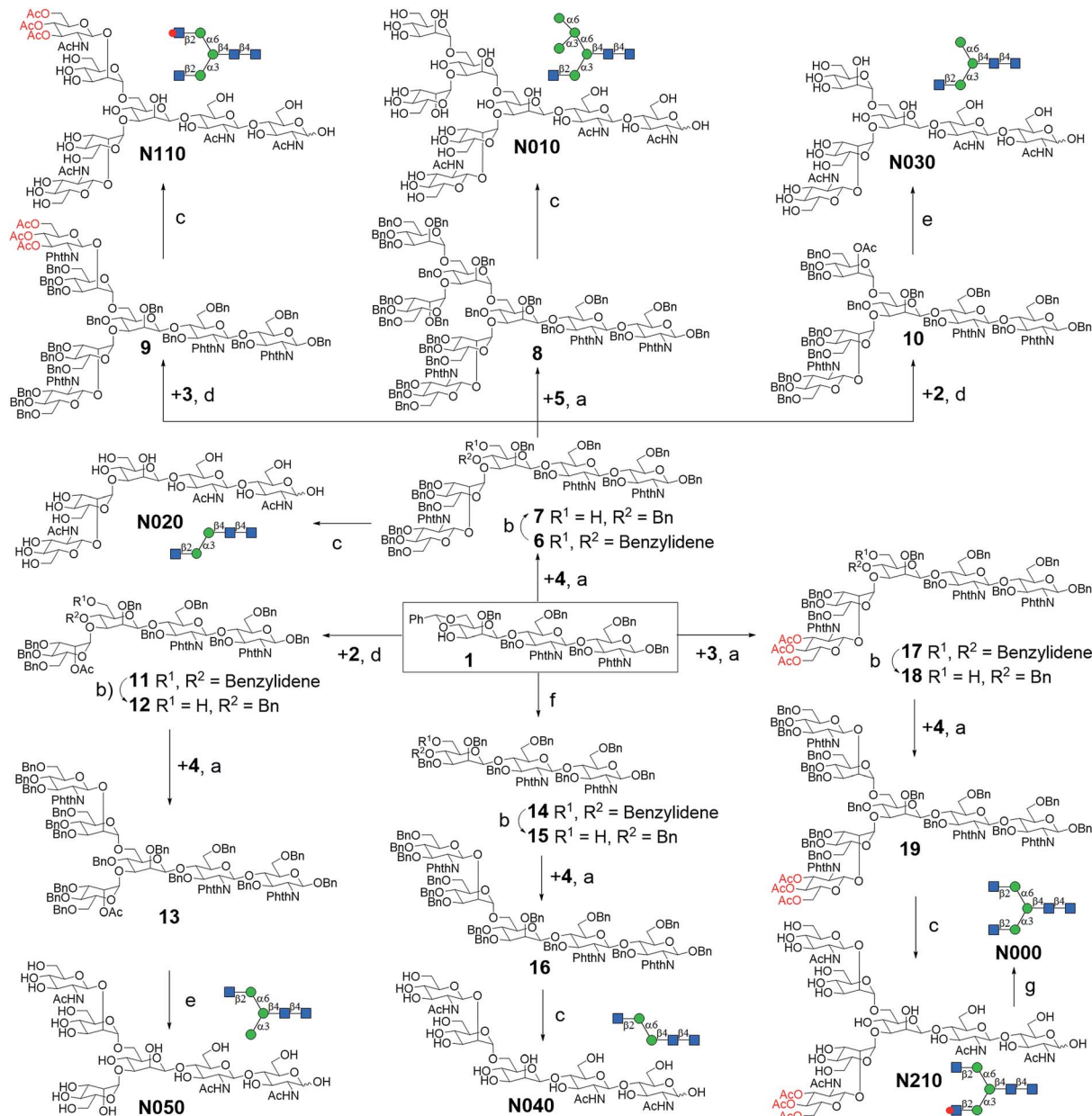
Scheme 1 Convergent synthesis of N-glycan core structures. Reagents and conditions: (a) NIS, AgOTf, Et 2 O, 0 °C, 6: 93%; 8: 85%; 9: 83%; 13: 90% ( \alpha/\beta = 5 : 1 ); 16: 91% ( \alpha/\beta = 3.5 : 1 ); 17: 94%; 19: 86% ( \alpha/\beta = 4 : 1 ); (b) PhBCl 2 , Et 3 SiH, DCM, -78 °C, 7: 96%; 12: 92%; 15: 95%; 18: 93%; (c) (1) ethylenediamine, n -butanol, 90 °C; (2) Ac 2 O, pyridine, rt; (3) Pd(OH) 2 , H 2 , MeOH/H 2 O (10 : 1), over three steps, N010: 63%; N020: 67%; N040: 61%; N110: 69%; N210: 65%; (d) NIS, AgOTf, DCM, 0 °C, 10: 91%; 11: 95%; (e) (1) ethylenediamine, n -butanol, 90 °C; (2) Ac 2 O, pyridine, rt; (3) NaOMe, MeOH; (4) Pd(OH) 2 , H 2 , MeOH/H 2 O (10 : 1), over four steps, N030, 53%; N050: 55%; (f) BnBr, NaH, DMF, 90%; (g) 30% NH 4 OH : H 2 O (1 : 10), quant.
