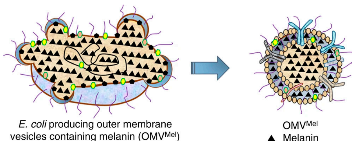
Figure 6. Scheme of the formation of OMVMel (OMV is outer membrane vesicle): OMVMel is purified after vesiculation from the parental bacteria. Reproduced from [116], with permission from Springer Nature, 2019.
