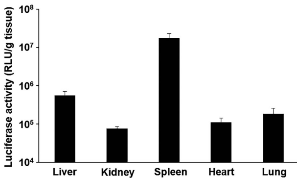
Figure 4. Transgene efficiency of the ternary complex in mice. Mice were intravenously administrated the ternary complex containing pCMV-Luc. Six hours after its administration, luciferase activities in the liver, kidneys, spleen, heart, and lungs were evaluated. Each bar was the mean \pm S.E.
