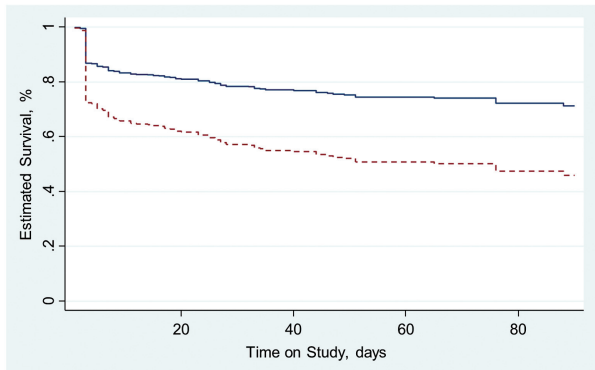
Fig. 4 Adjusted estimated survival curves according to the original JAAM and modified JAAM-2 DIC status using the FORECAST dataset. (A) JAAM DIC score \leq 3 , (B) JAAM DIC score \geq 4 , (C) JAAM-2 DIC score \leq 2 , and (D) JAAM-2 DIC score \geq 3 . The solid line represents patients in the anticoagulant group, and the dotted line represents patients in the control group. DIC, disseminated intravascular coagulation; JAAM, Japanese Association for Acute Medicine.
