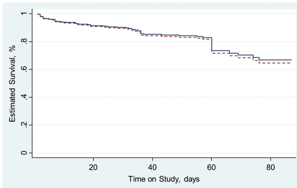
Fig. 4 Adjusted estimated survival curves according to the original JAAM and modified JAAM-2 DIC status using the FORECAST dataset. (A) JAAM DIC score \leq 3 , (B) JAAM DIC score \geq 4 , (C) JAAM-2 DIC score \leq 2 , and (D) JAAM-2 DIC score \geq 3 . The solid line represents patients in the anticoagulant group, and the dotted line represents patients in the control group. DIC, disseminated intravascular coagulation; JAAM, Japanese Association for Acute Medicine.
