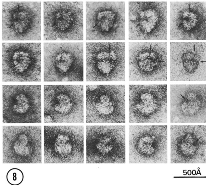
FIGURE 8 Selected images of cytoribosomes. The images of the first row and the first two images of the second row are left-featured; the last three images of the second row are right-featured frontal images. The third row shows right-lateral, and the fourth row left-lateral images. The vertical arrows (first and second row) point to the partition in the small subunit. The horizontal and oblique arrows point to the dense spot located between the subunits in frontal images or in front of the small subunit in lateral images. The horizontal dense band between large and small subunit is clearly visible in the right featured frontal images. \times 400,000 .
