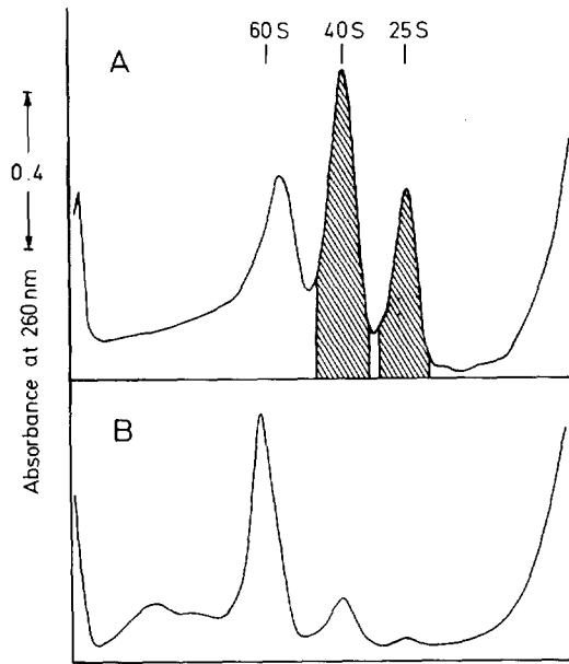
FIGURE 2 Gradient profiles of fixed mitochondrial ribosomes. The ribosomes were prepared after lysis of mitochondria in 0.055 M MgCl_2 ; the gradients contained no magnesium. The shadowed areas represent material used for electron microscopy. (A) Ribosomes were resuspended in 0.004 M EDTA before treatment with glutaraldehyde. (B) Ribosomes were resuspended in AMT before treatment with glutaraldehyde.
