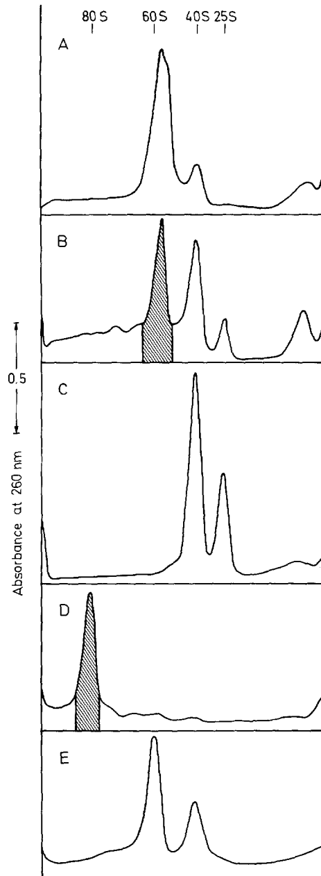
FIGURE 1 Gradient profiles of unfixed mitochondrial and cytoplasmic ribosomes. The shaded areas represent material used for electron microscopy. (A) Mitochondrial ribosomes prepared after lysis of mitochondria in AMT (magnesium containing gradient). (B) Mitochondrial ribosomes prepared after lysis of mitochondria in 0.055 M MgCl_2 (magnesium containing gradient). (C) Mitochondrial ribosomes prepared after lysis of mitochondria in 0.055 M MgCl_2 (magnesium-free gradient). (D) Cytoplasmic ribosomes (magnesium containing gra-
