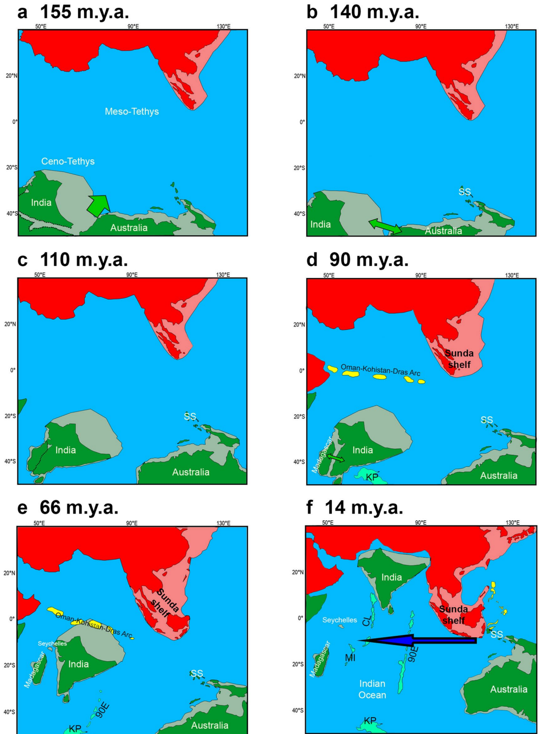
Figure 1. Geologic reconstruction of the Indian Ocean’s continents through the Mesozoic and part of the Cenozoic at 155 Ma (a), 140 Ma (b), 110 Ma (c), 90 Ma (d), 66 Ma (e), and 14 Ma (f). Laurasian landmasses are represented in red and Gondwanan landmasses in green. Areas in yellow are volcanic islands and in cyan are volcanic ridges (90E: Ninetyeast Ridge; CL: Chagos-Laccadive Ridge; MI: Mascarene Islands) and plateaus (KP: Kerguelen Plateau). The lightly coloured areas next to the continents represent continental shelves, which may or may not have been emergent depending on the timeframe. Dashed lines represent boundaries of continental break-ups; green arrows represent major break-up events; and the blue arrow represents the MIOJet. SS: Sula Spur. Redrawn from refs. 1,5,8 .
