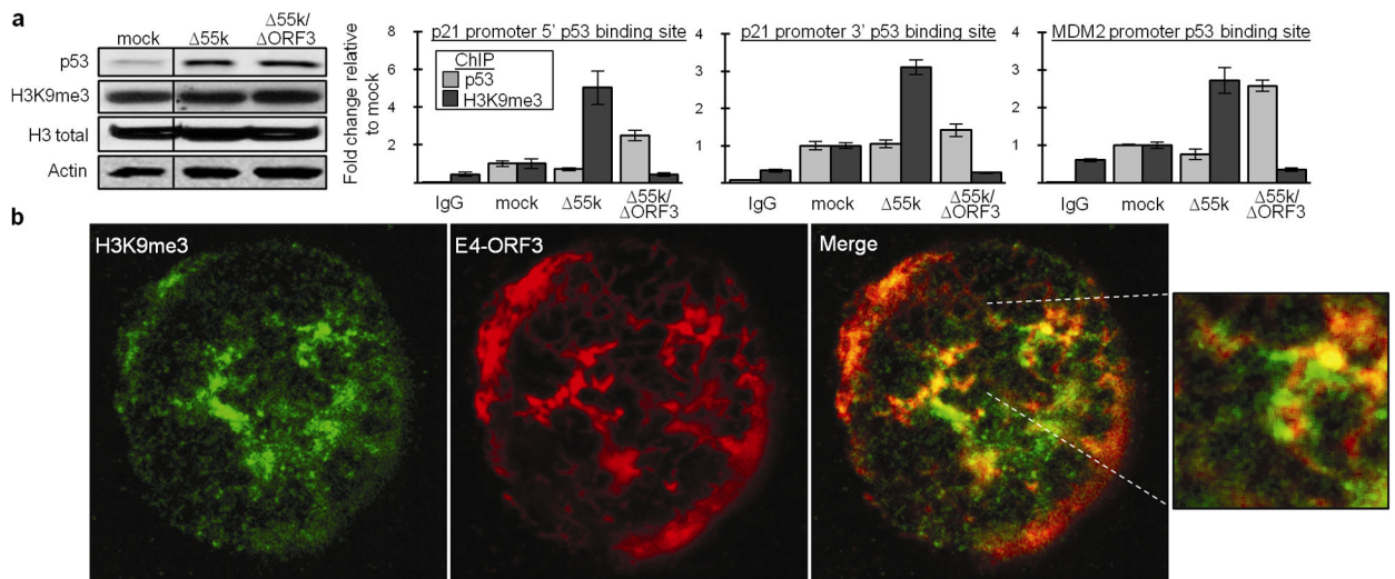
Fig 4. E4-ORF3 forms a nuclear scaffold that specifies heterochromatin assembly and H3K9 trimethylation at p53 target promoters
