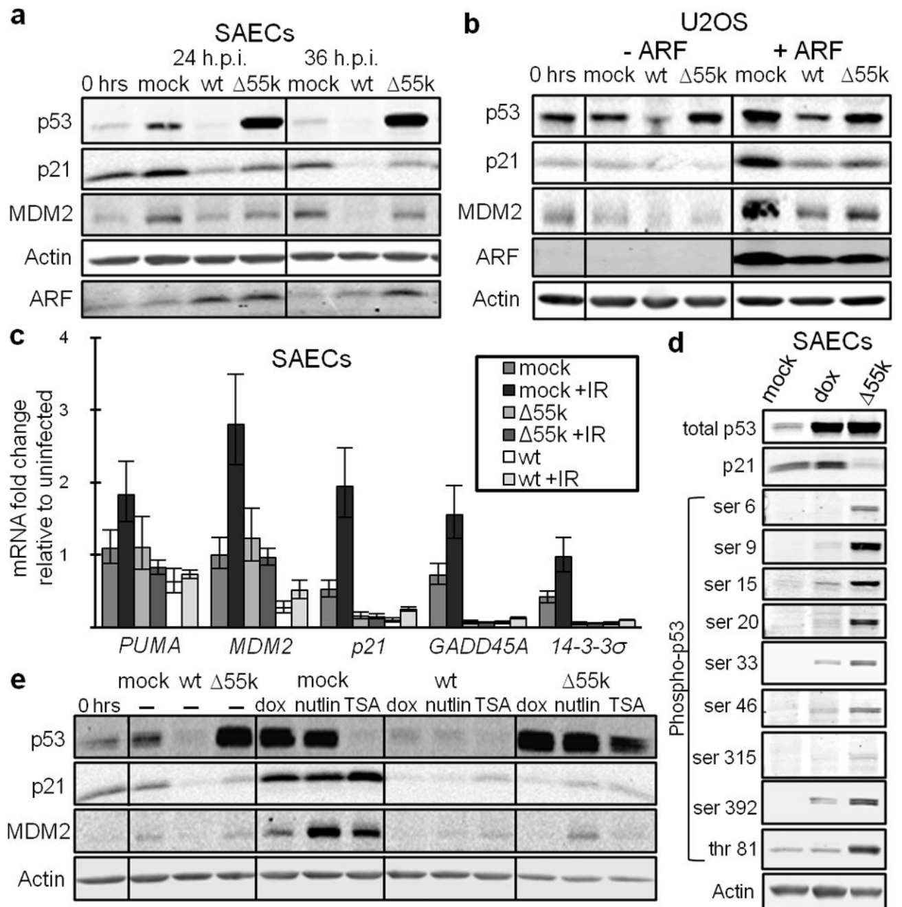
Fig 1. p53 is induced and phosphorylated in E1B-55k infection but p53 activity is dominantly suppressed
