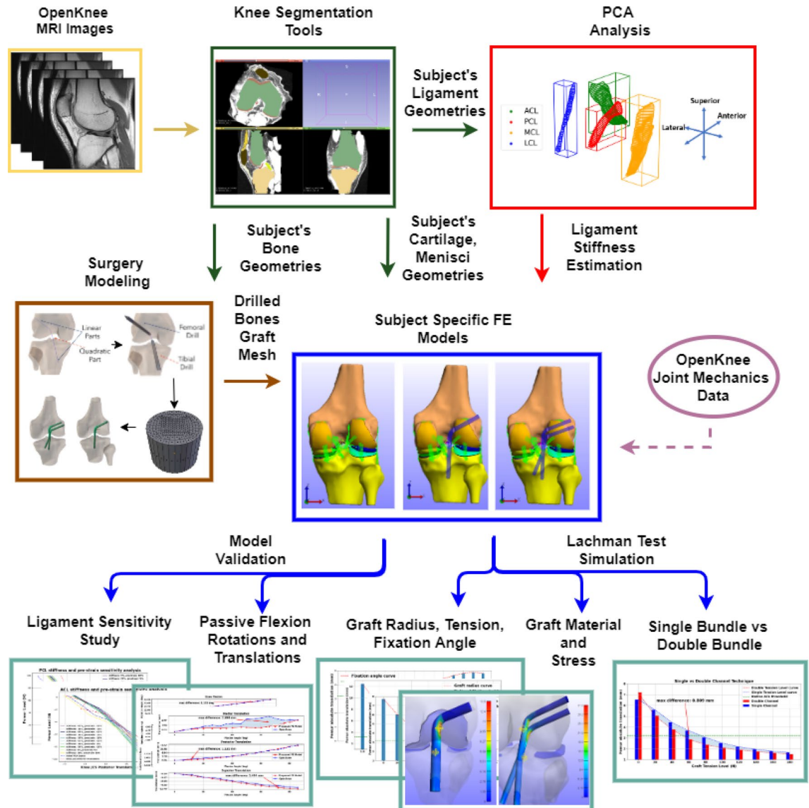
Figure 1. Overview of the proposed workflow. MRI data are used to propose a surgery plan for subject-specific ACLR. First, we use open-source segmentation tools to acquire geometries of the anatomical structures. Next, PCA is applied to ligament geometries to acquire subject-specific estimation of stiffness (PCA block). The bone geometries are used in the Surgery Modeling tool to drill the tunnels. During this process, the graft mesh is also generated. Subsequently, we automatically generate FE models of the knee joint. Joint mechanics data from the open-source Open Knee(s) project are used to develop and validate a RM. Then, the surgery parameters are evaluated by performing a FE simulation of the Lachman clinical examination. The performance of models that correspond to the ACL reconstructed knee joint are compared to that of the RM. The measurements of interest are relative knee displacement and graft maximum principal stress (Diagrams.net, v17.2.1, https://www.diagrams.net/ ).
