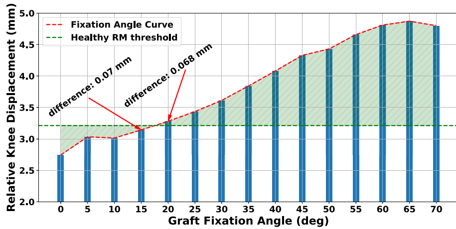
Figure 9. Effect of graft fixation angle on relative knee displacement. The “difference” term refers to the absolute difference in relative knee displacement between the ACLR FE model and the RM. It is noticed that for angles larger than 30° the relative knee laxity increases. In our case, we found the optimal fixation angles are between 15° and 20°.
