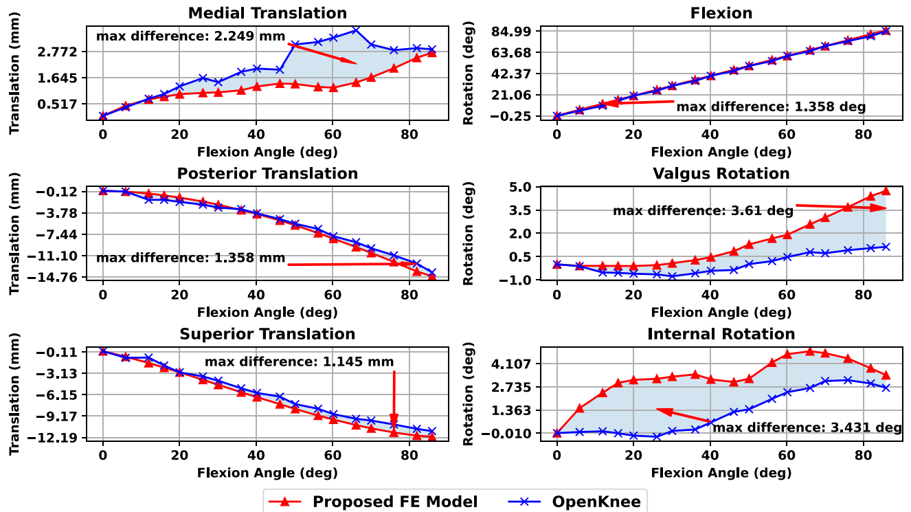
Figure 6. Comparison of simulated and experimental kinematics during passive knee flexion (translations left and rotations right). We observe that the proposed FE model exhibits comparable performance for the translations except for the medial-lateral direction. Regarding rotations, different behavior is evident for the internal-external rotation with a good initial match during varus-valgus rotation.
