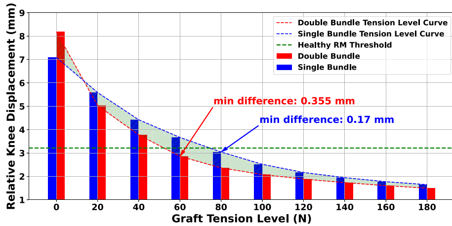
Figure 10. Results for comparing the SB and DB techniques. The “difference” term refers to the absolute difference in relative knee displacement translation between the FE model and the RM. Although the DB method appears to be superior in restraining knee laxity, the margin between the two methods is not disproportionate.
