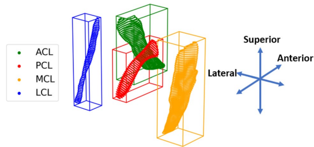
Figure 4. Estimating ligament stiffness from MRI. Cross-sections and the bounding box of each ligament surface mesh are presented. Multiple cross-sections are taken along the principal ligament axis derived by PCA. The ligament's cross-sectional area is estimated as the mean of the areas of each slice.
