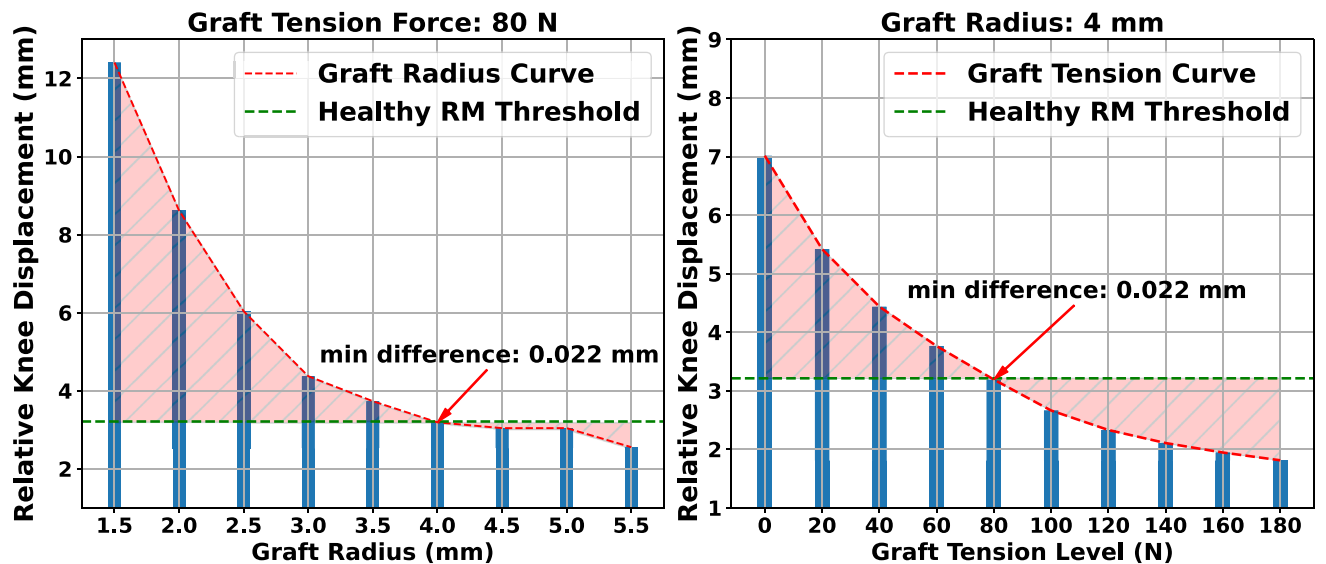
Figure 7. Effect of graft radius and pretension on knee laxity for a semitendinosus graft. The “difference” term refers to the absolute difference in relative knee displacement between each ACLR FE model and the RM. Increasing the graft radius for a specific pretension load reduces relative displacement. The same applies when increasing graft pretension for a fixed value of graft radius.
