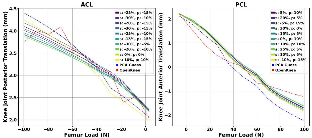
Figure 5. Aggregated results from the sensitivity analysis with the ten best combinations of stiffness and prestrain values for ACL and PCL. The estimated stiffness (PCA method) and recommended prestrain value from Blakenvoort were used as initial guesses. The “s” and “p” denote the stiffness and prestrain percentage change, respectively. In addition, we observed combinations that include the initial stiffness value and changed only the prestrain by a factor.
