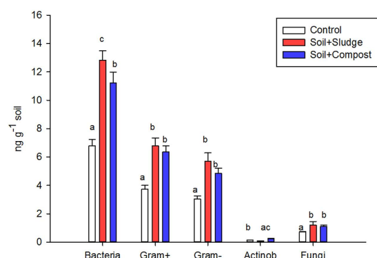
Figure 1. PLFA content of different microbial groups in control and restored plots. Data followed by the same letter are not significantly different according to the HSD test ( P < 0.05 ). Actinob = Actinobacteria.
