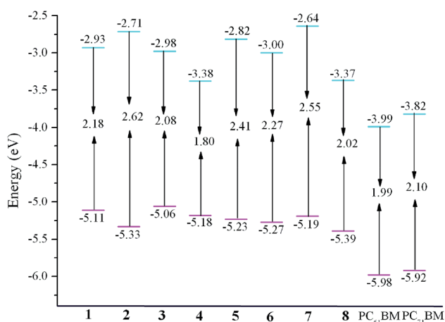
Fig. 2 Evaluation of calculated FMO energies for investigated molecules as well as FMO energies for PC 61 BM and PC 71 BM at the PBE0/6-31G(d,p) level.
