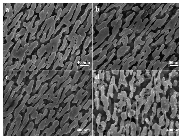
Fig. 10 SEM images of NR substrate. (a) Ag@Au NR array substrate before \text{H}_2\text{O}_2 treatment. (b) Ag@Au NR array substrate after \text{H}_2\text{O}_2 treatment. (c) AgNR substrate before \text{H}_2\text{O}_2 treatment. (d) AgNR substrate after \text{H}_2\text{O}_2 treatment.
