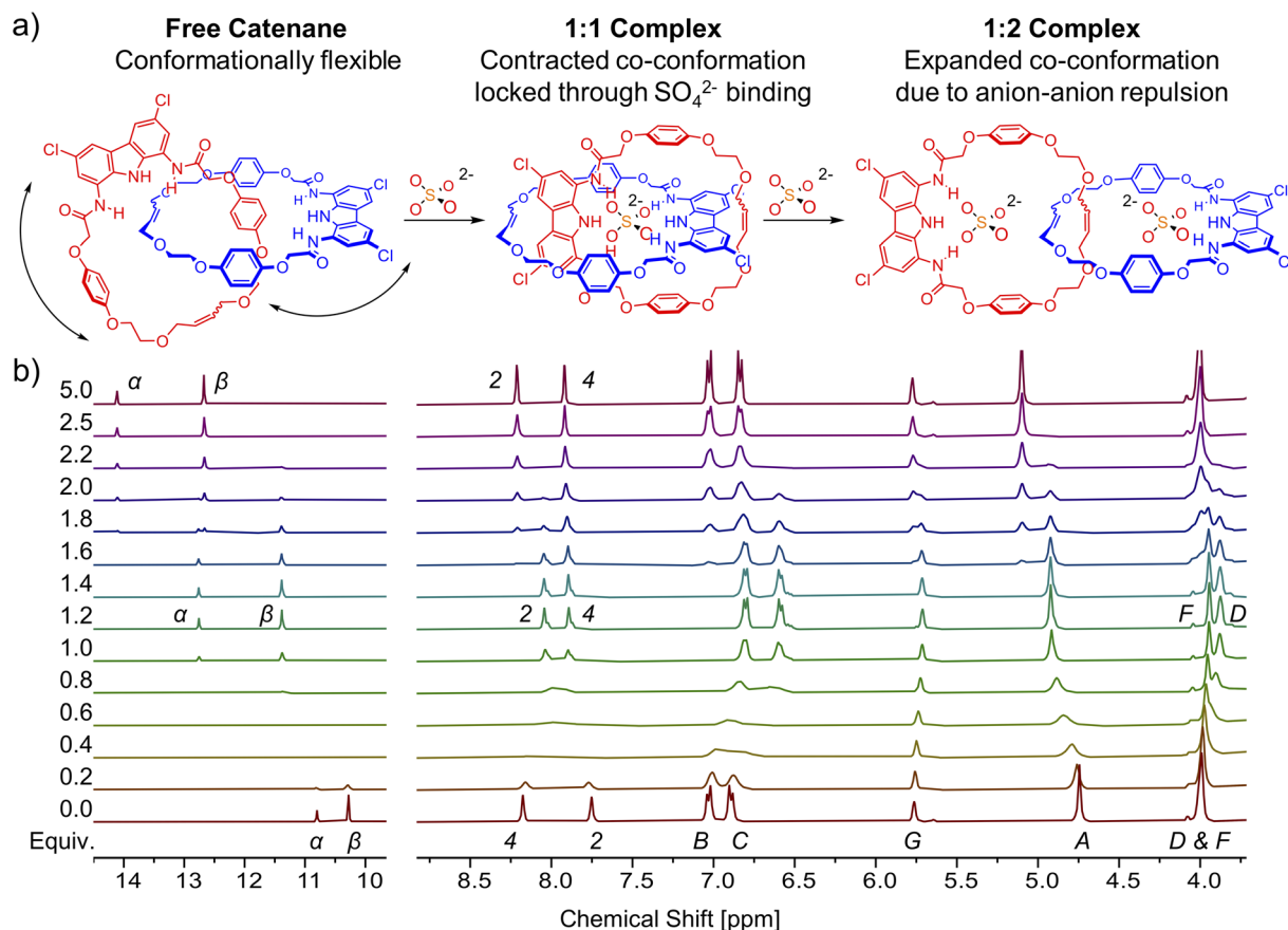
Fig. 5 (a) Graphical representation of the complexes formed during the titration of [2]catenane A with TBA 2 SO 4 . (b) Truncated 1 H NMR spectra of [2]catenane A with increasing amount of TBA 2 SO 4 in DMSO- d 6 + 0.5% H 2 O.
