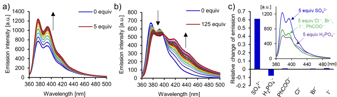
Fig. 9 Emission spectra recorded during titration of [2]catenane A with TBA_2SO_4 (a) and TBAH_2PO_4 (b) in DMSO/H_2O 9 : 1 (ex: 350 nm). (c) Relative change of emission intensity: (I - I_0)/I_0 of catenane A at 370 nm in the presence of 5 equiv. of TBA salts. Inset: comparison of emission spectra of [2]catenane A in the presence of 5 equiv. of TBA salts of SO_4^{2-} , H_2PO_4^- , PhCOO^- , and halides ( Cl^- , Br^- , and I^- ) in DMSO/H_2O 9 : 1 (ex: 350 nm).
