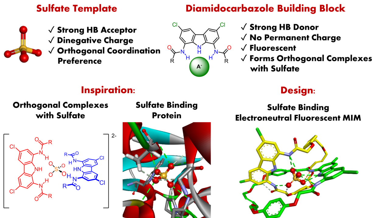
Fig. 1 Sulfate template and high affinity diamidocarbazole building blocks enable the synthesis of the electroneutral fluorescent [2]catenane, capable of binding sulfate inside an interlocked hydrogen bonding cavity reminiscent of the binding site of Sulfate Binding Protein (SBP).
