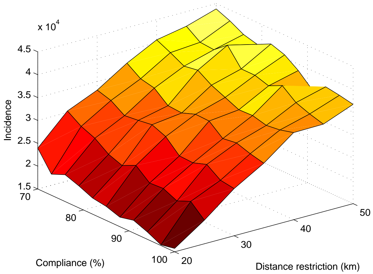
Figure 4 Total incidence for varying compliance and restrictions. A surface plot showing incidence after 60 days with the parameters of compliance and distance restrictions on the data axes. 1000 realizations were made for each point. The surface has its highest values at high set distance limit and low compliance. Its low values are found at opposite corner.
