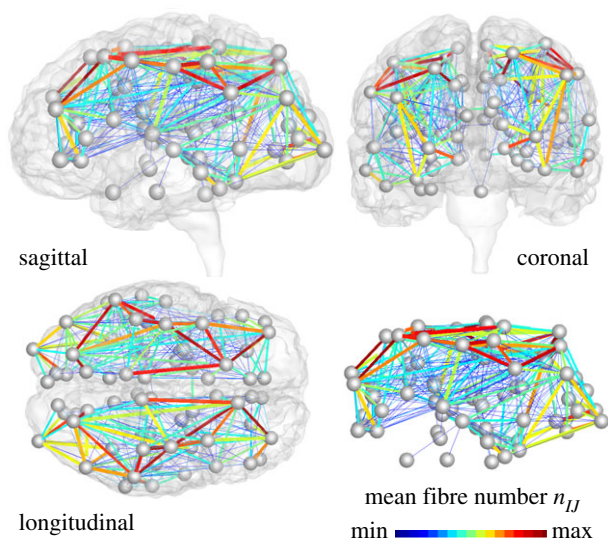
Figure 5. Brain network model. Misfolded tau proteins spread across the brain's connectome represented as a weighted graph \mathcal{G} with N = 83 nodes and E = 1130 edges. Edges are weighted by the mean fibre number n_{ij} divided by the mean fibre length l_{ij} averaged over 418 healthy brains from the Human Connectome Project. (Online version in colour.)
