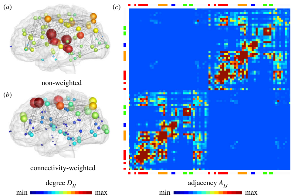
Figure 6. Brain network model. The connectivity of the graph \mathcal{G} is represented through the degree D_{II} , the number of edges per node, and the adjacency A_{IJ} = n_{IJ}/l_{IJ} , the ratio of fibre number and length. (a) Degree D_{II} of non-weighted and (b) connectivity-weighted graphs and (c) adjacency A_{IJ} of connectivity-weighted graph, averaged over 418 healthy brains from the Human Connectome Project. (Online version in colour.)
