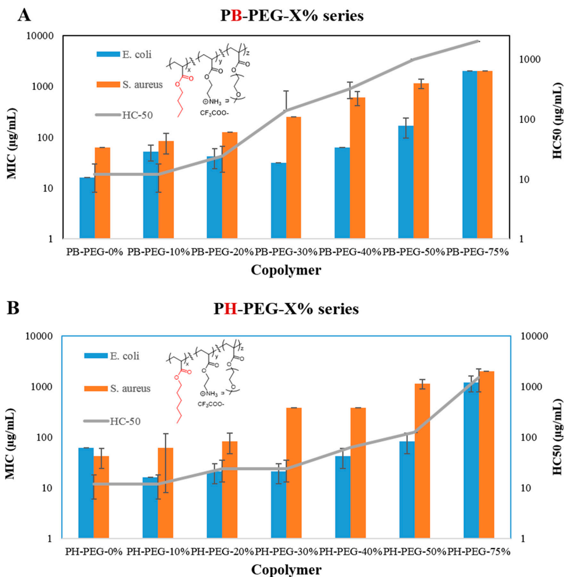
Figure 2. Antibacterial (MIC) and hemolytic activities (HC 50 ) of (A) PB-PEG-X% series, terpolymers of butyl acrylate (shown in red in structure), 2-(( tert -butoxycarbonyl)amino)ethyl acrylate, and PEGMA-300; (B) PH-PEG-X% series, terpolymers of hexyl acrylate (shown in red in structure), 2-(( tert -butoxycarbonyl)amino)ethyl acrylate, and PEGMA-300. Error bars represent standard deviation.
