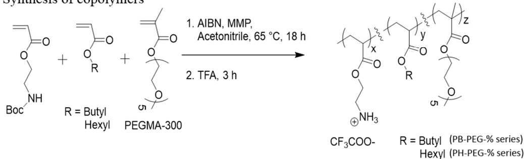
(B) Synthesis of copolymers
