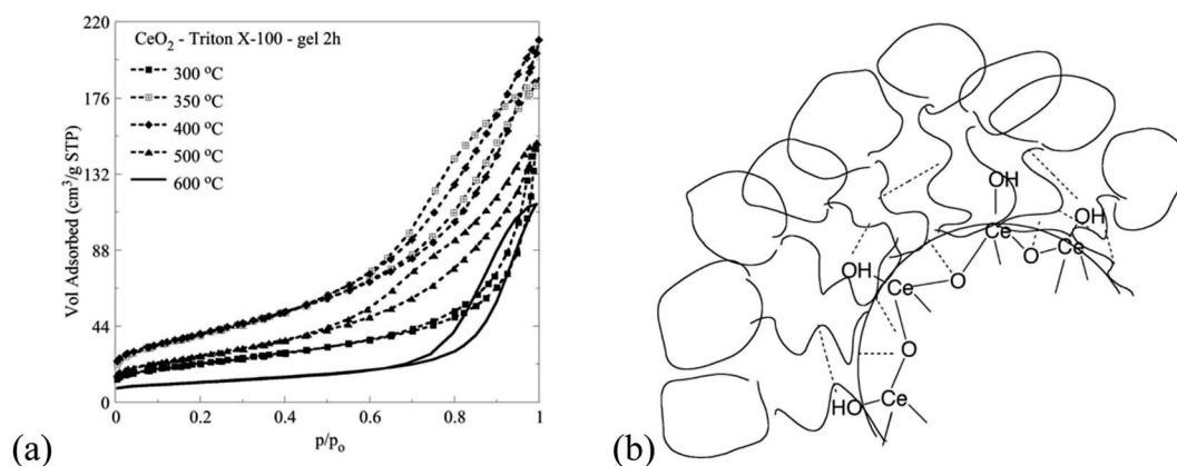
Fig. 9 N_2 ad/desorption isotherms of ceria particles corresponding to Triton X-100 after direct calcination at different temperatures (a) and schematic illustration of possible interactions between the Triton X-100 polar tails and the ceria precursors (b).
