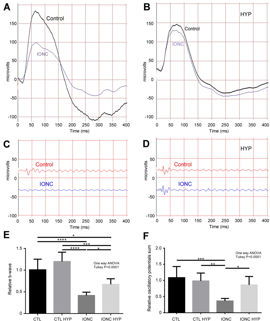
Figure 1. Representative electroretinograms showing the a- and b-waves (A,B) and the oscillatory potentials (C,D) of the right (sham-operated, control) and the left (IONC) eye of experimental rats kept at room temperature (A,C) or subjected to therapeutic hypothermia (B,D). Quantification of the relative (left eye/right eye) b-waves (E) and oscillatory potentials (F) are represented as histograms for the 4 experimental groups: sham-operated rats (CTL), sham rats treated with hypothermia (CTL HYP), rats subjected to IONC (IONC), and animals subjected to IONC and treated with hypothermia (IONC HYP). Bars represent the mean \pm SD of all samples ( n = 10 animals per group). Asterisks represent statistically significant differences. * p < 0.05 ; ** p < 0.01 ; *** p < 0.001 ; **** p < 0.0001 .
