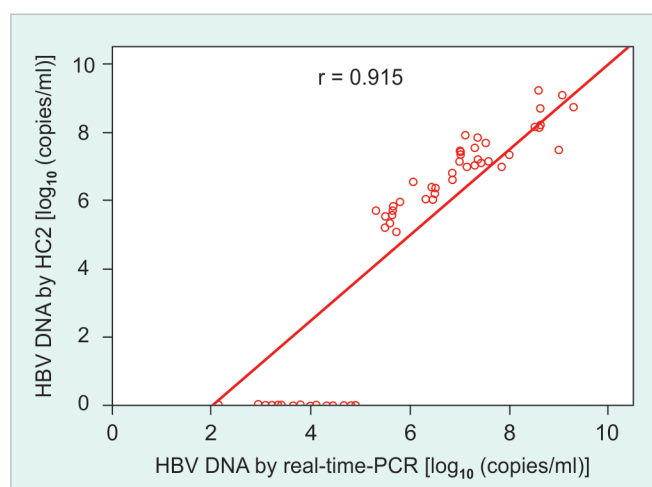
Fig. 1: A log-log plot of hepatitis B virus DNA concentrations in 66 samples as measured by real-time-polymerase chain reaction and HC2 assay. Strong correlation ( r = 0.915 ) was observed between results obtained with the two assays for the 40 concordant positive samples. A total of 26 samples tested negative by HC2 assay, but 20 of these had detectable hepatitis B virus DNA by real-time-PCR, while six samples had undetectable DNA by both the assay
