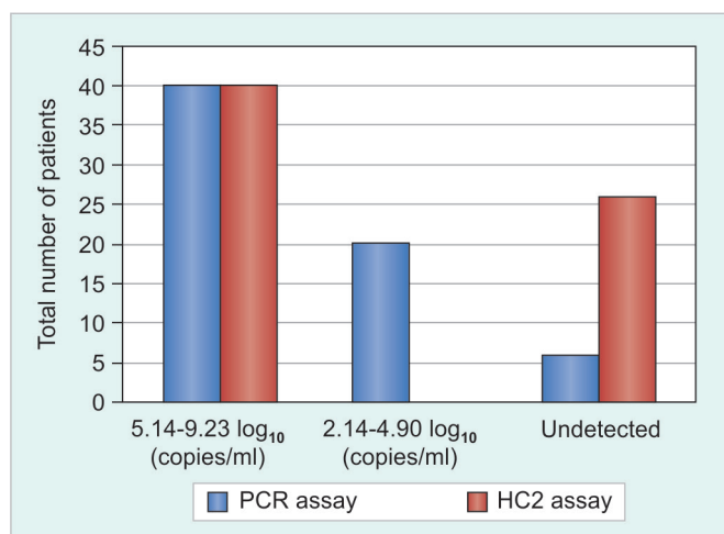
Fig. 2: Comparison between real-time-polymerase chain reaction and HC2 assay for HBV DNA detection
