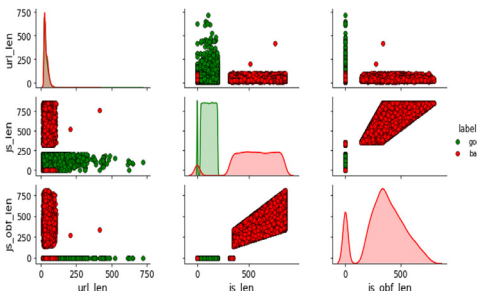
Fig. 9. Trivariate pairwise plot.
