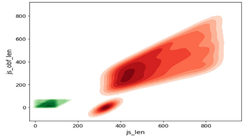
Fig. 12. Bivariate density plot.
