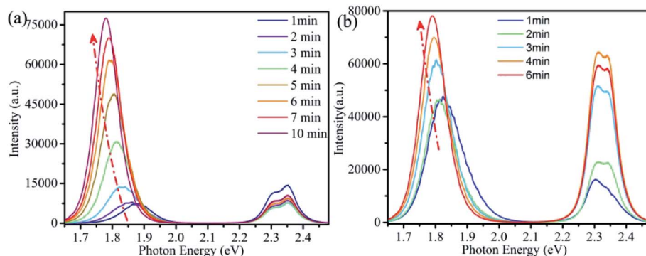
Fig. 2 (a) PL spectra evolution of a single \text{CsPbBr}_x\text{I}_{3-x} microsheel with the irradiation time of CW laser (wavelength \lambda = 355 nm and power P = 0.2 mW). (b) PL spectra of the same \text{CsPbBr}_x\text{I}_{3-x} microsheel after stored in desiccator for 72 h.
