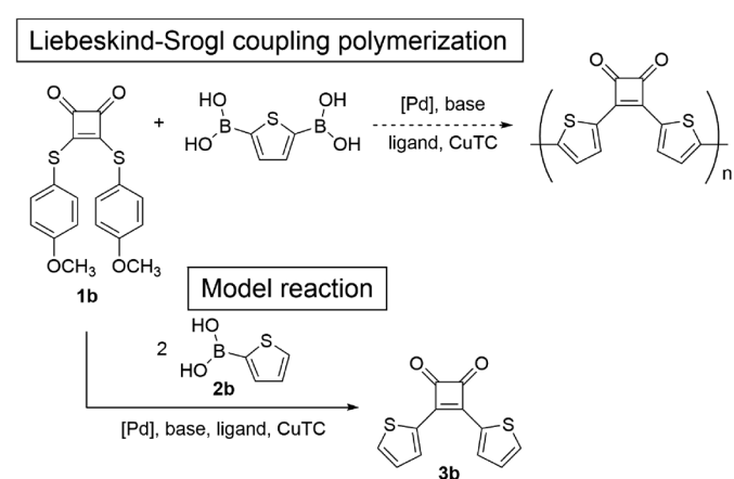
Scheme 2 Model reaction for the direct Liebeskind–Srogl coupling polymerization of 3,4-bis[(4-methoxyphenyl)thio]-3-cyclobutene-1,2-dione ( 1b ) and 2,5-thiophenediboronic acid.
