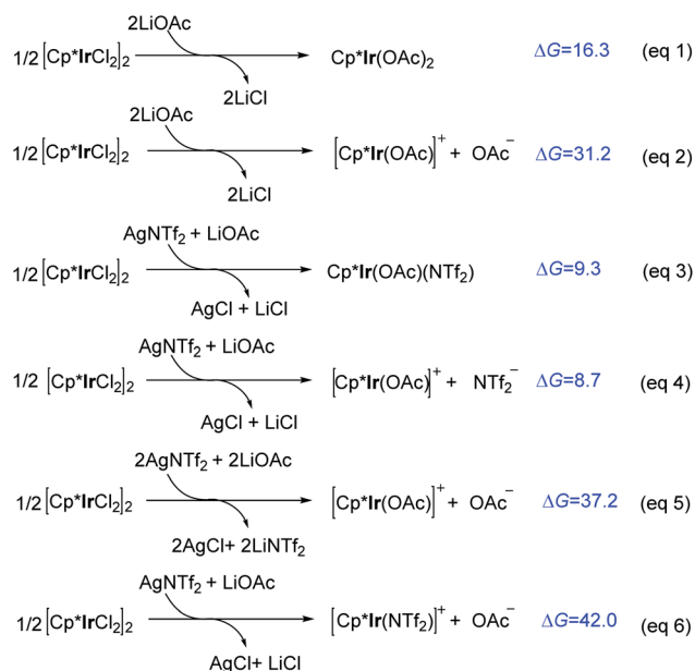
Scheme 3 Calculated reaction free energies ( \Delta G , kcal mol −1 ) for the formation of various Ir(III) species.
