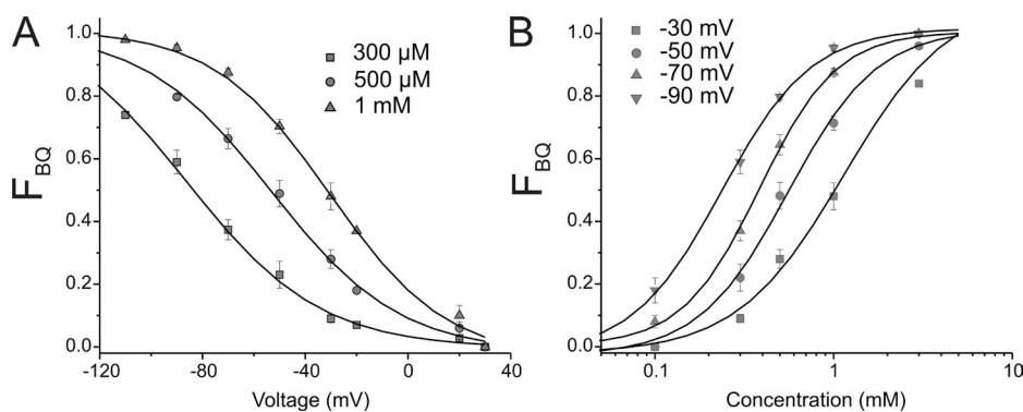
Figure 6. Concentration and voltage dependence of the inhibition of single Cx50 hemichannels by BQ + applied to the extracellular side. (A) Plots of fractional inhibition (F BQ ) versus V m at BQ + concentrations of 300 μM, 500 μM, and 1 mM demonstrate the voltage dependence of inhibition. Solid lines are fits to a Boltzmann equation. The mean V 1/2 values from Boltzmann analysis are -86, -53, and -30 mV, with slope factors of 26, 25, and 23 mV -1 for 300 μM, 500 μM, and 1 mM BQ + , respectively. (B) Plots of fractional inhibition (F BQ ) versus BQ + concentrations of -30, -50, -70, and -90 mV. The solid lines are fits to the Hill equation, with K d values of 1.14, 0.556, 0.38, and 0.24 mM and Hill slopes of 1.6, 1.7, 1.9, and 1.7 at -30, -50, -70, and -90 mV, respectively.
