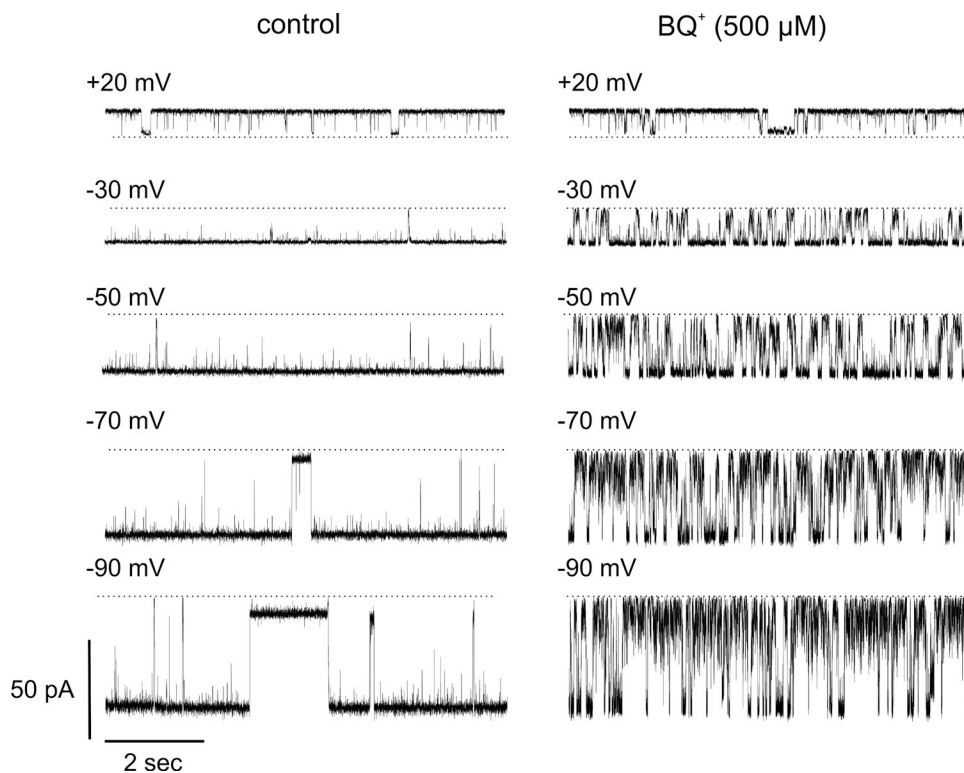
Figure 5. Voltage-dependent inhibition of Cx50 hemichannels by extracellular BQ + suggests a binding site in the pore. Recordings of single-hemichannel currents in excised patches in control (left) and in 500 μM BQ + (right) at membrane potentials of +20, -30, -50, -70, and -90 mV are shown. BQ + was applied to the extracellular side of the hemichannel. Dashed lines in the current traces indicate the closed state. In the absence of BQ + , Cx50 hemichannels predominantly reside in the open state at voltages between +20 and -70 mV. With further hyperpolarization, Cx50 hemichannels tend to gate to long-lived sub-conductance states (see trace at -90 mV). The application of 500 μM BQ + to the extracellular side caused strong hyperpolarizing inhibition at large hyperpolarizing voltages, but little inhibition at smaller hyperpolarizing voltages (compare P o in BQ + at -30 and -90 mV). An increase in inhibition with hyperpolarization, which tends to drive BQ + into the hemichannel, is suggestive of a binding site within the aqueous pore.
