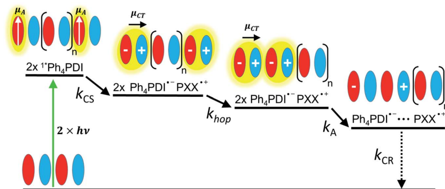
Fig. 1 CT biexciton annihilation model. Following photoexcitation, two photons create two singlet Frenkel excitons on \text{Ph}_4\text{PDI} acceptor molecules, which then rapidly charge separate to create two CT excitons with a rate constant of k_{\text{CS}} . The transition dipole moment of \text{Ph}_4\text{PDI} , \mu_{\text{A}} , is perpendicular to the CT exciton transition dipole moment, \mu_{\text{CT}} . CT exciton migration with a site-to-site rate constant, k_{\text{hop}} , and collision result in CT biexciton annihilation, which produces spatially separated electron–holes pairs with a rate constant k_{\text{A}} . Alternatively, the CT biexciton can be produced on adjacent D–A pairs resulting in annihilation. The electron–hole pair recombination rate is k_{\text{CR}} .
