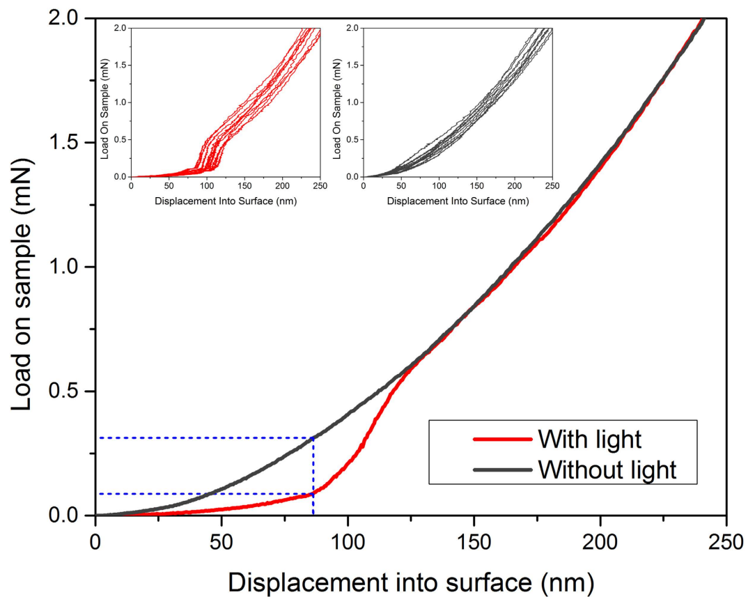
Figure 2. Nanoindentation loading curves (average curves, n = 10 ) for hydrophilic sample (single crystal gold), with and without 670 nm laser. The force required for the diamond tip to penetrate \sim 100 nm into the metal is less when the tip/substrate contact zone is irradiated. Insets display the corresponding measurements shown as individual curves. Representative curves for single crystal aluminum have been presented during the International Conference on Laser Applications in Life Sciences, 2014 40 .
